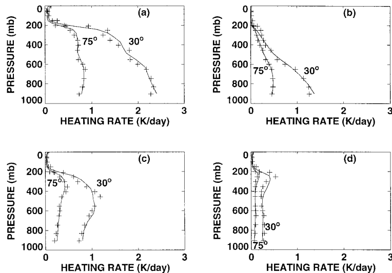
FIG. 1. Comparisons of the heating rate profiles computed with the LBL method (solid) and k -distribution functions from Table 1 (pluses) taking into account the solar radiation absorption due to the water vapor lines and continuum. Calculations were performed for the midlatitude summer atmosphere and for the two solar zenith angles 30^\circ and 75^\circ in the spectral intervals (a) from 0.7 to 5 \mu\text{m} , (b) from 0.7 to 1.22 \mu\text{m} , (c) from 1.22 to 2.27 \mu\text{m} , and (d) from 2.27 to 5 \mu\text{m} .
